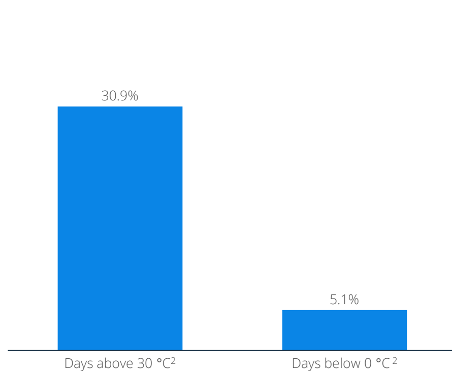
Shares of days with extreme temperatures yearly 1
